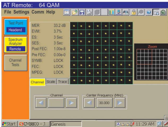
Upstream Constellation
